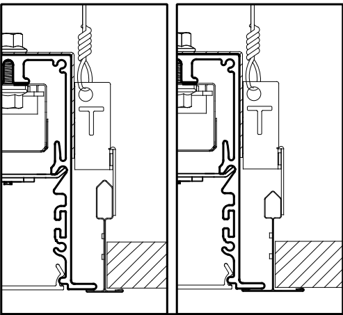
9/16 T-GRID 15/16 T-GRID
